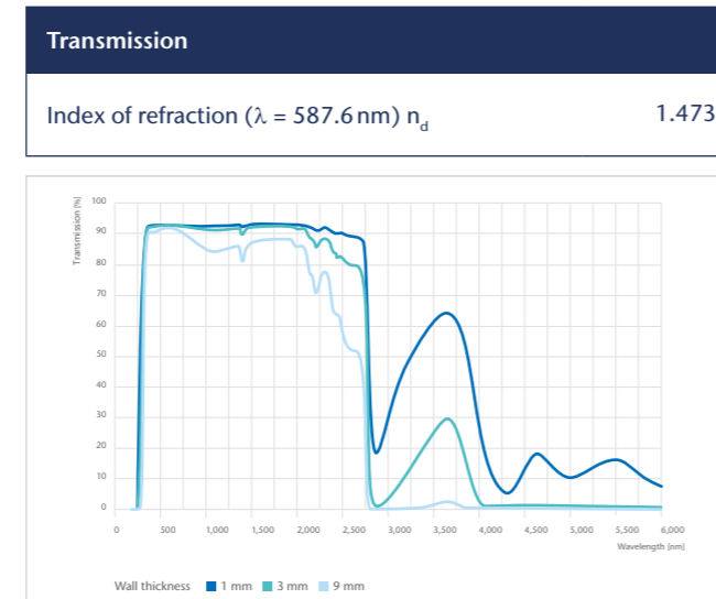
Transmission curves for WT of 1 mm, 3 mm, 9 mm
