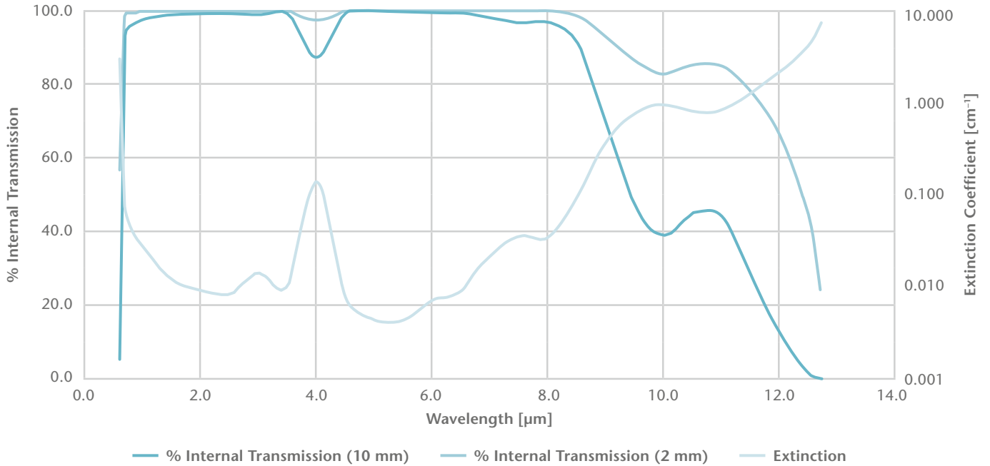
IRG 27 Extinction and Internal Transmission
